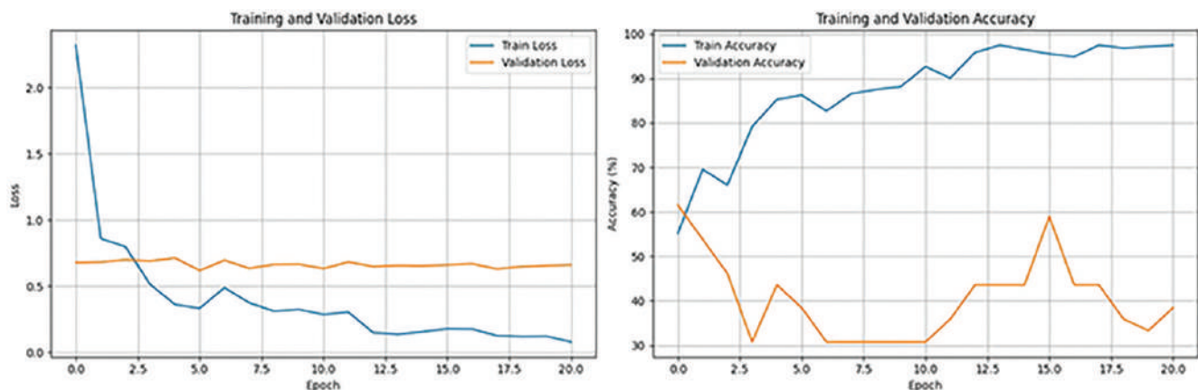
Figure 1. Training and validation accuracy.
