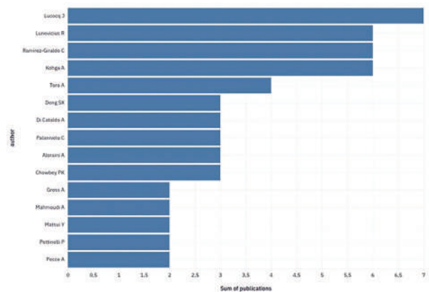
Figure 2. Top authors.
