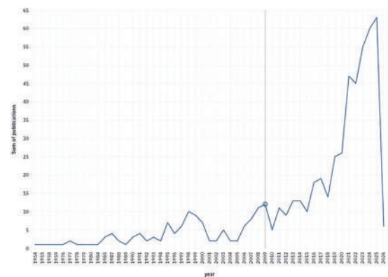
Figure 3. Publication trends.
