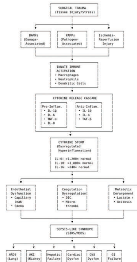
Figure 1. Etiopathogenesis of the cytokine storm.
