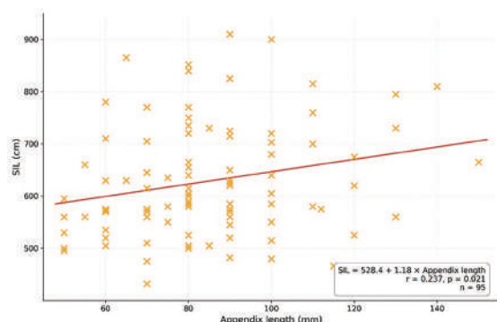
Figure 2. Correlation between small intestine length (SIL) and appendix length. Scatter plot illustrating the relationship between SIL and appendix length (n=95). The linear regression equation is SIL = 528.4 + 1.18 \times \text{appendix length (mm)} . The plot demonstrates a weak but statistically significant positive correlation ( r=0.237 , p=0.021 ).
