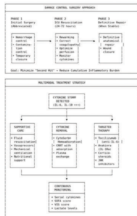
Figure 2. Treatment algorithms.
